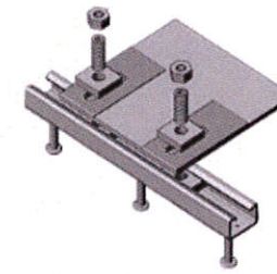
Anchorage channels for concrete
